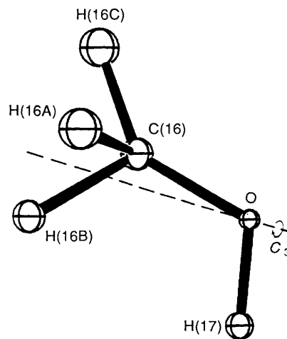
Fig. 3 An ORTEP plot 32 of the methanol molecule of solvation in \text{fac-}[\text{IrH}_3(\text{PPh}_2\text{Me})_3] . Only one of the three disordered orientations is shown
