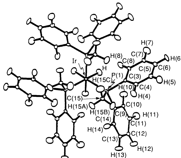
Fig. 2 Complete molecular plot of \text{fac-}[\text{IrH}_3(\text{PPh}_2\text{Me})_3]
