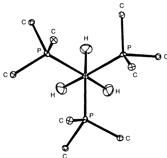
Fig. 1 An ORTEP plot 32 of the core of \text{fac-}[\text{IrH}_3(\text{PPh}_2\text{Me})_3] . A crystallographic three-fold rotational axis passes through the molecule
